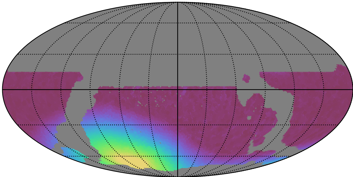
weather_cloudso35v3.4_10yrs WFD y band: Min moonDistance
