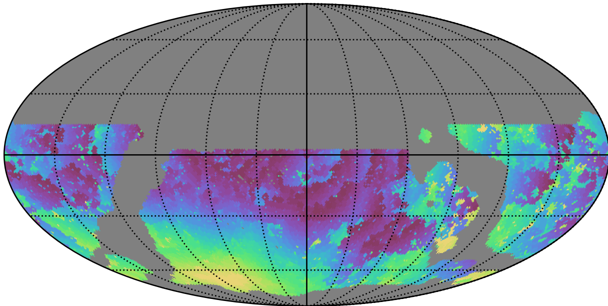
weather_cloudso35v3.4_10yrs WFD u band: Min moonDistance
