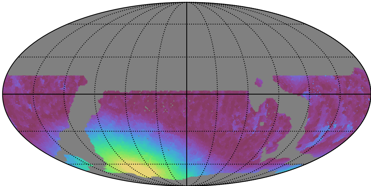
weather_cloudso35v3.4_10yrs WFD r band: Min moonDistance
