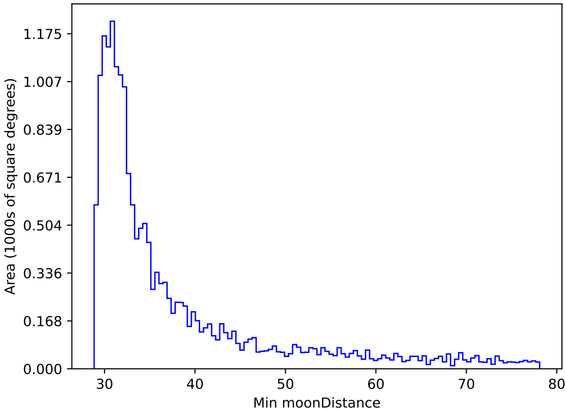
weather_cloudso35v3.4_10yrs WFD r band: Min moonDistance
