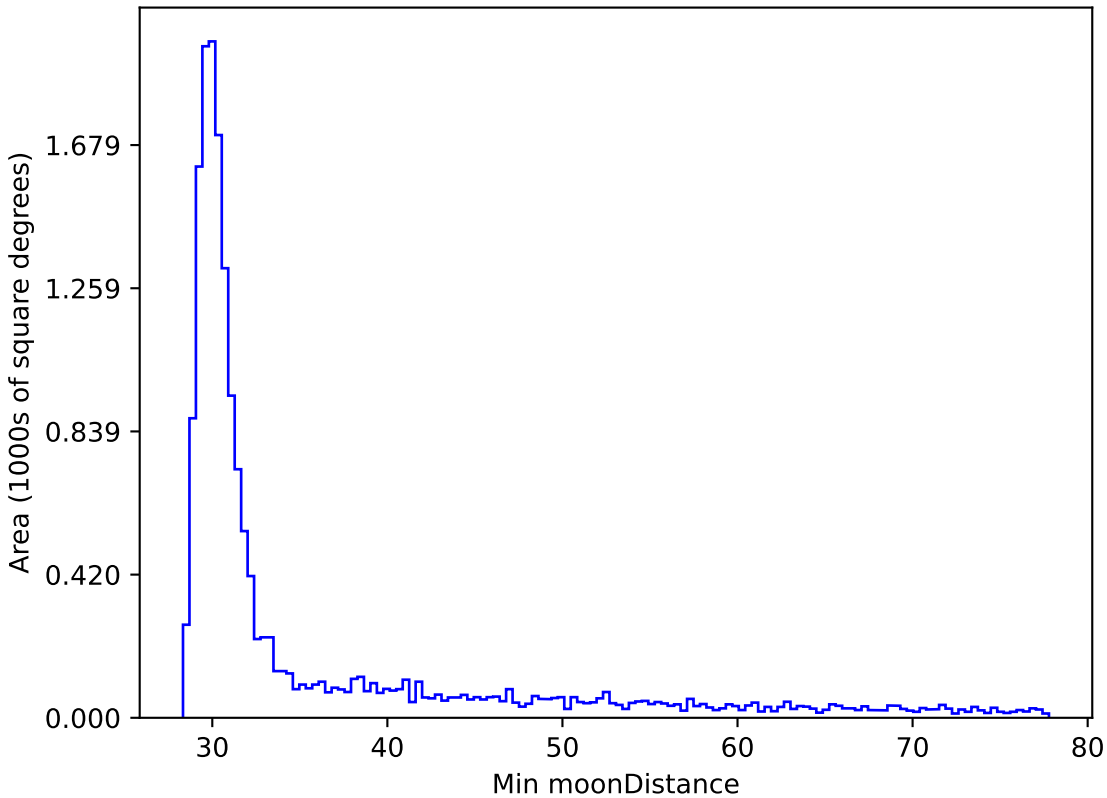
weather_cloudso35v3.4_10yrs WFD i band: Min moonDistance
