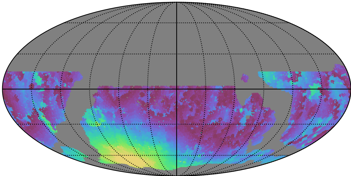
weather_cloudso35v3.4_10yrs WFD g band: Min moonDistance
