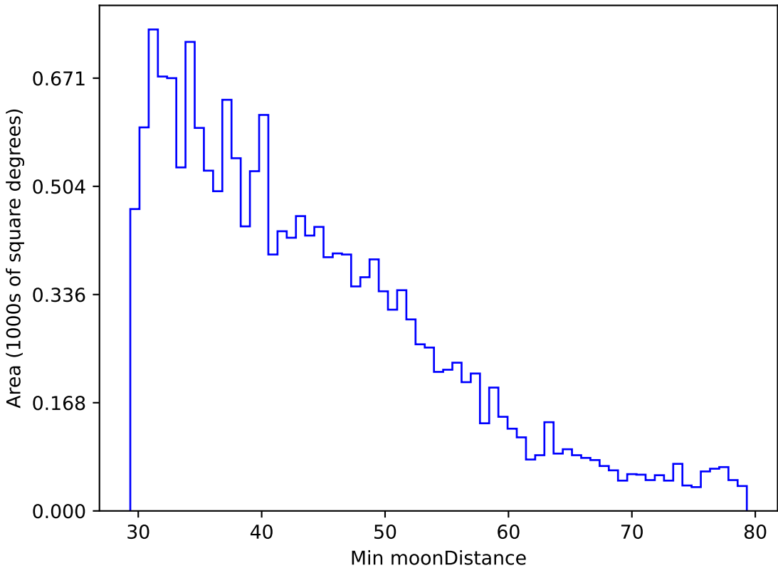
weather_cloudso35v3.4_10yrs WFD g band: Min moonDistance
