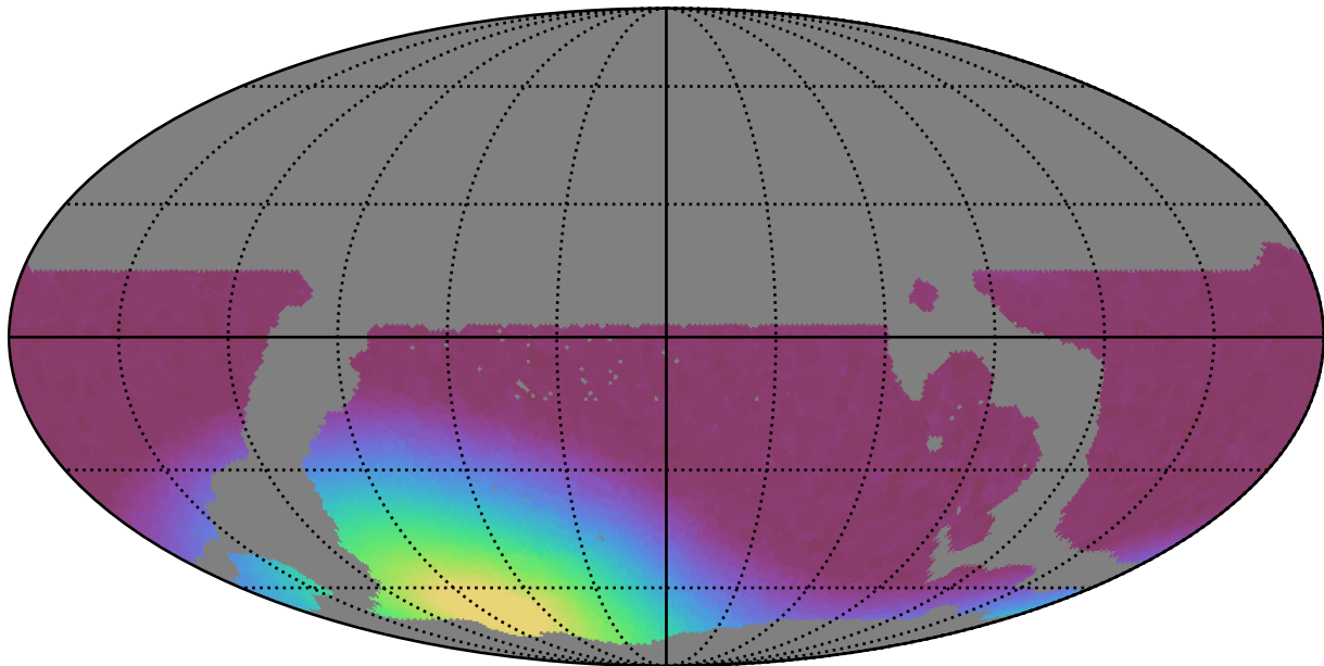
weather_cloudso35v3.4_10yrs WFD all bands: Min moonDistance
