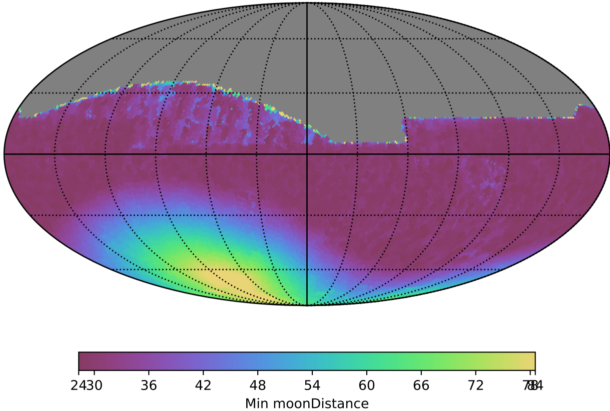
weather_cloudso35v3.4_10yrs All sky z band: Min moonDistance
