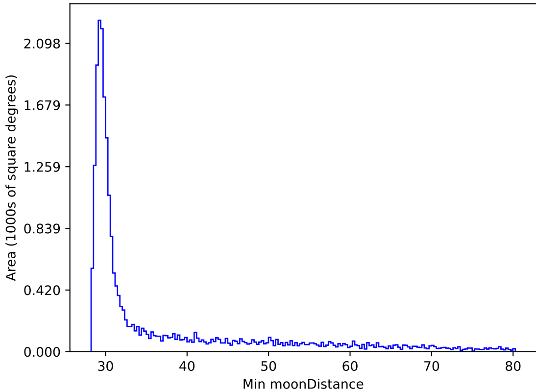
weather_cloudso35v3.4_10yrs All sky y band: Min moonDistance
