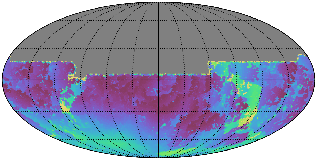
weather_cloudso35v3.4_10yrs All sky u band: Min moonDistance
