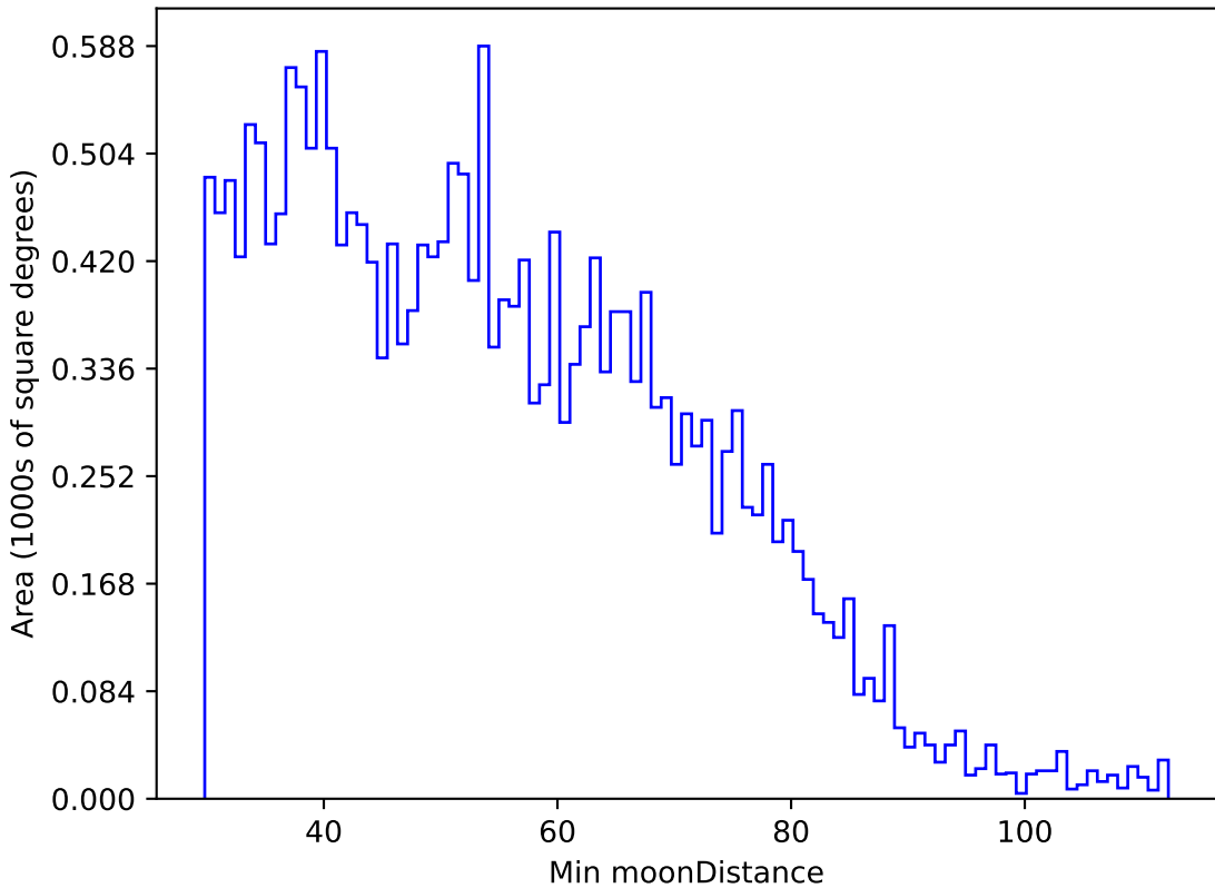
weather_cloudso35v3.4_10yrs All sky u band: Min moonDistance
