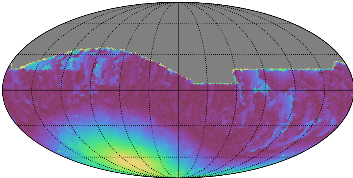
weather_cloudso35v3.4_10yrs All sky r band: Min moonDistance
