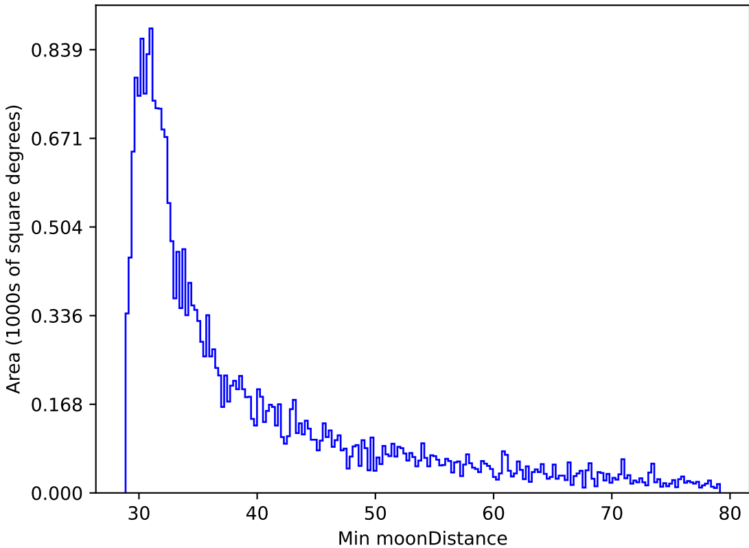
weather_cloudso35v3.4_10yrs All sky r band: Min moonDistance
