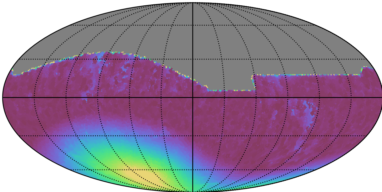
weather_cloudso35v3.4_10yrs All sky i band: Min moonDistance
