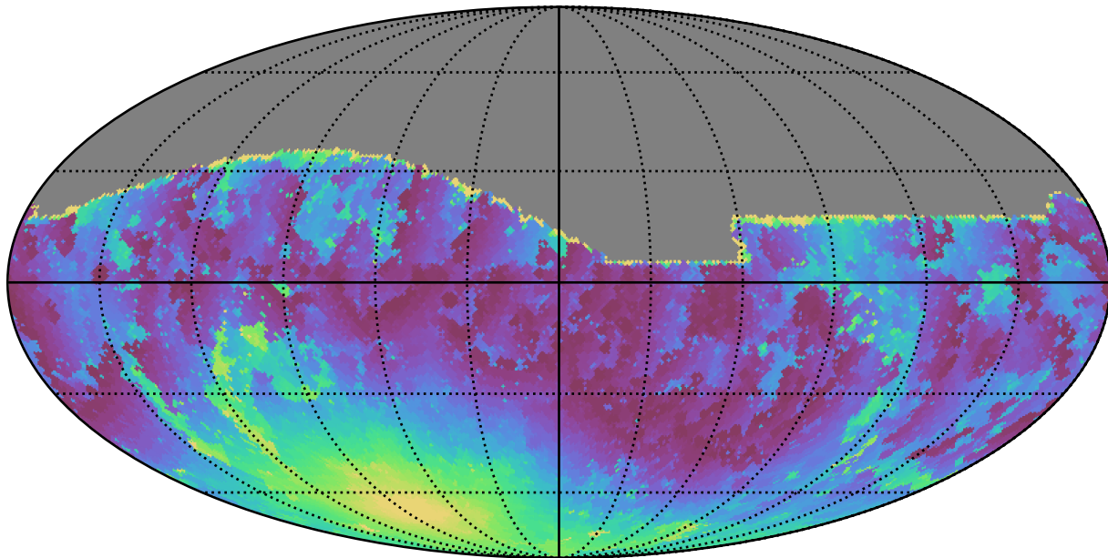
weather_cloudso35v3.4_10yrs All sky g band: Min moonDistance
