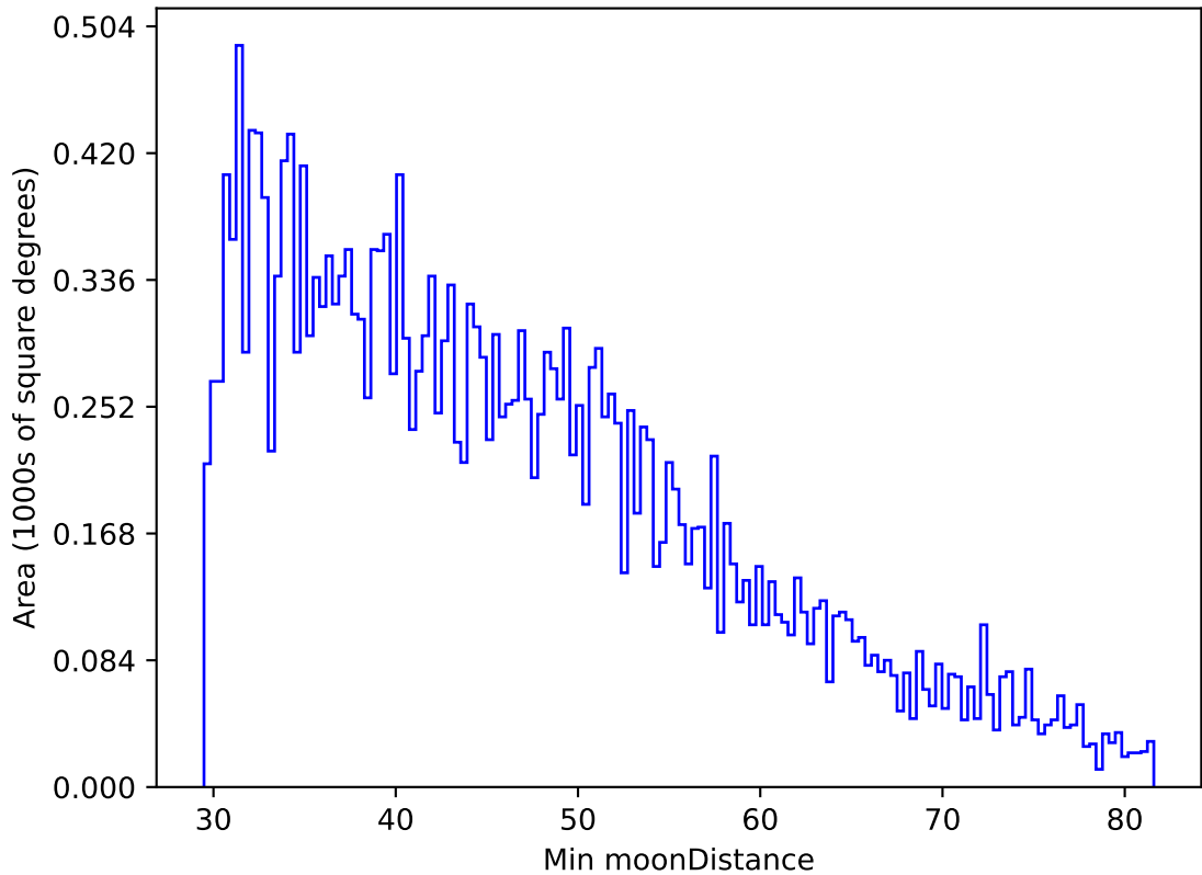
weather_cloudso35v3.4_10yrs All sky g band: Min moonDistance
