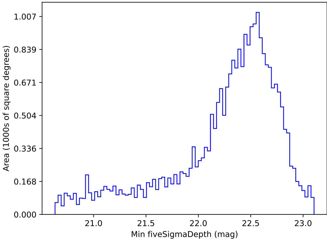
weather_cloudso35v3.4_10yrs Yr 1 z band: Min fiveSigmaDepth
