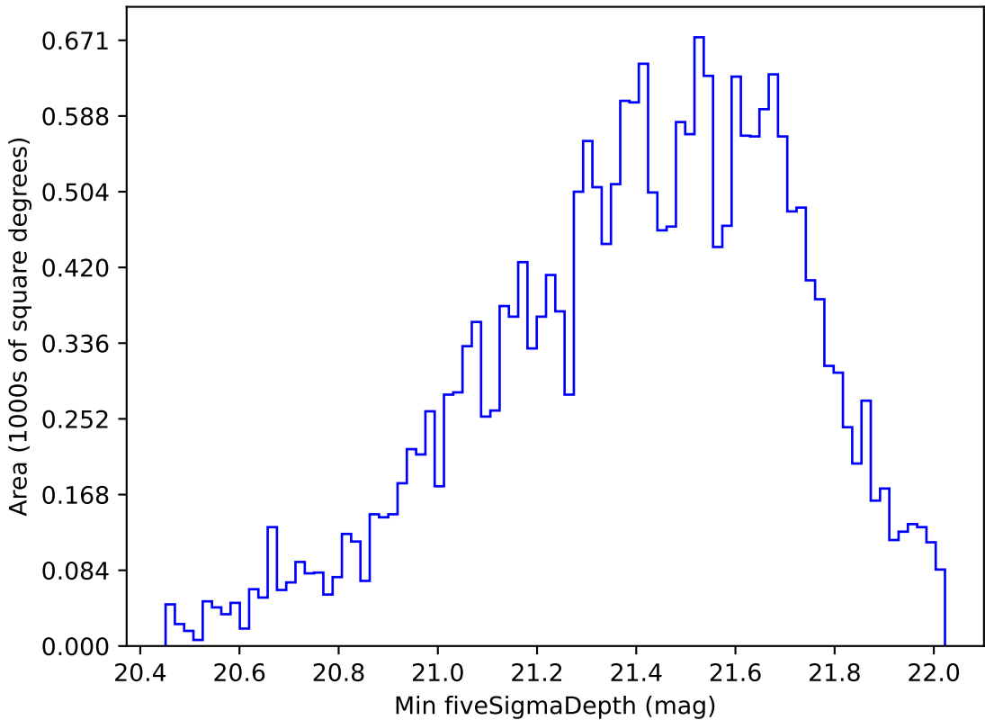
weather_cloudso35v3.4_10yrs Yr 1 y band: Min fiveSigmaDepth
