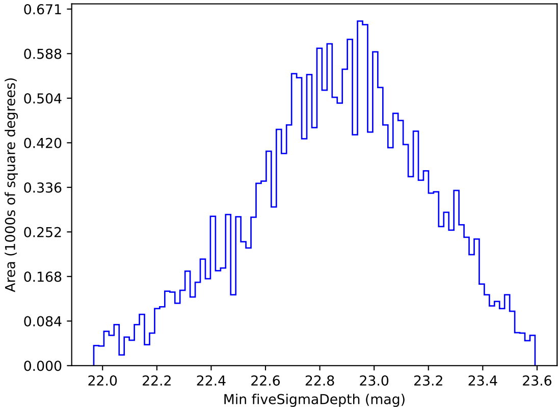
weather_cloudso35v3.4_10yrs Yr 1 u band: Min fiveSigmaDepth
