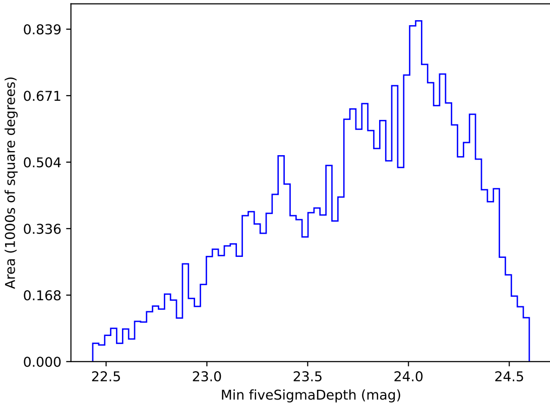
weather_cloudso35v3.4_10yrs Yr 1 g band: Min fiveSigmaDepth
