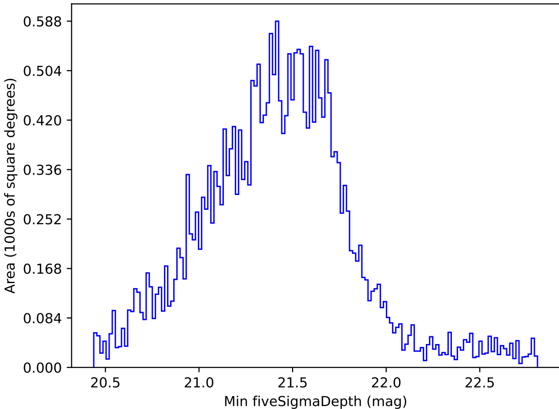
weather_cloudso35v3.4_10yrs Yr 1 all bands: Min fiveSigmaDepth
