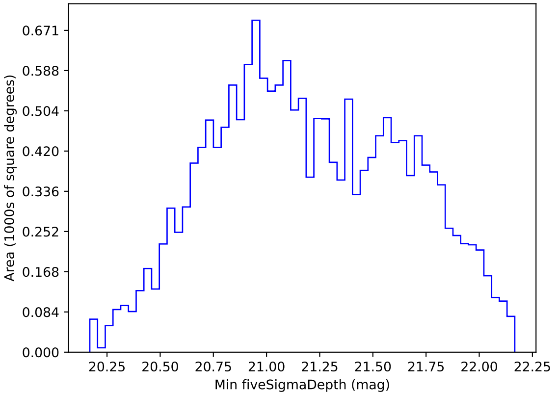
weather_cloudso35v3.4_10yrs WFD z band: Min fiveSigmaDepth
