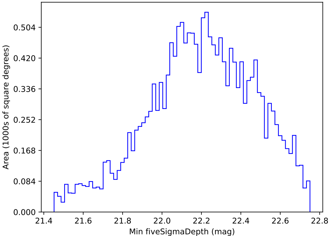
weather_cloudso35v3.4_10yrs WFD u band: Min fiveSigmaDepth
