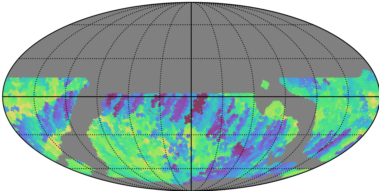
weather_cloudso35v3.4_10yrs WFD r band: Min fiveSigmaDepth
