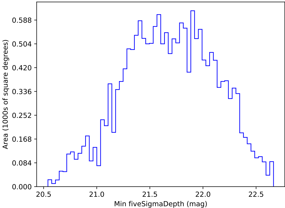
weather_cloudso35v3.4_10yrs WFD i band: Min fiveSigmaDepth
