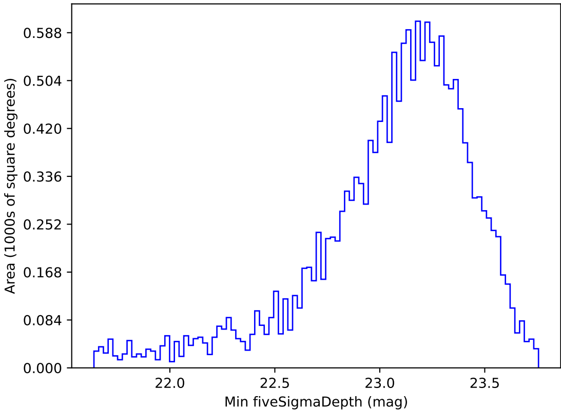
weather_cloudso35v3.4_10yrs WFD g band: Min fiveSigmaDepth
