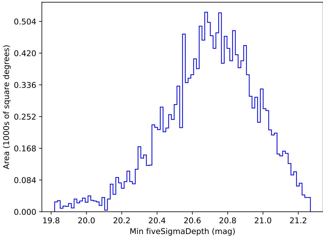
weather_cloudso35v3.4_10yrs WFD all bands: Min fiveSigmaDepth
