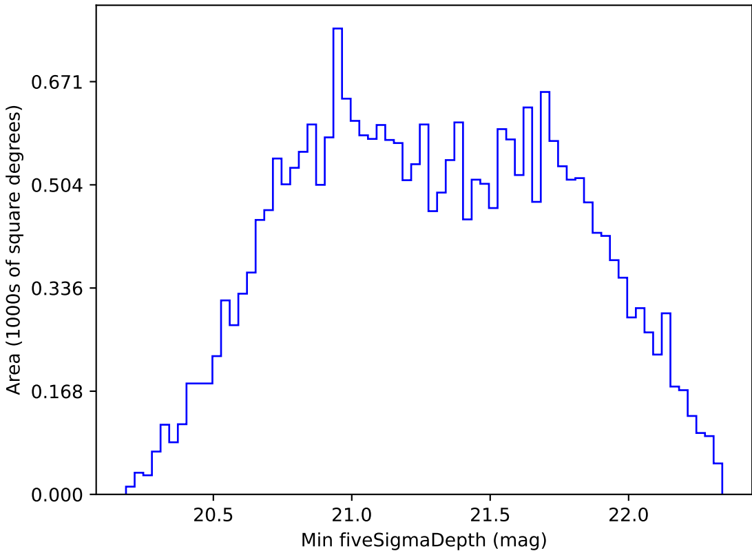
weather_cloudso35v3.4_10yrs All sky z band: Min fiveSigmaDepth
