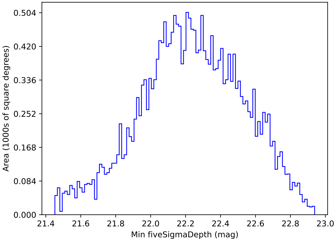
weather_cloudso35v3.4_10yrs All sky u band: Min fiveSigmaDepth
