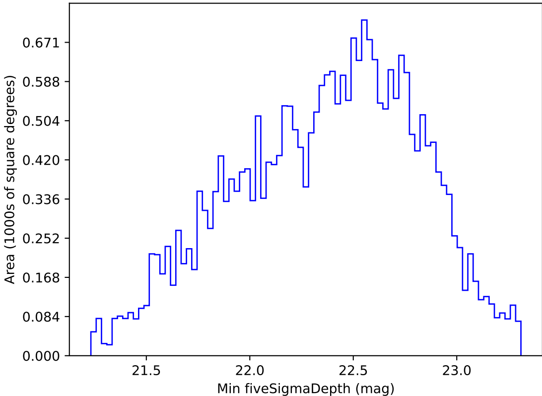
weather_cloudso35v3.4_10yrs All sky r band: Min fiveSigmaDepth
