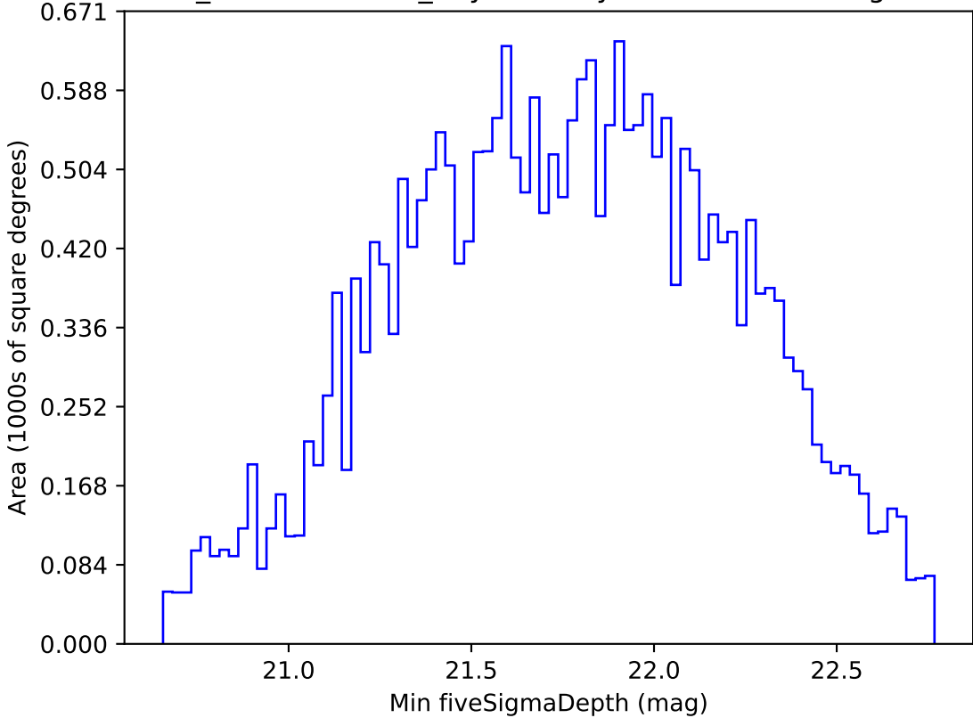
weather_cloudso35v3.4_10yrs All sky i band: Min fiveSigmaDepth
