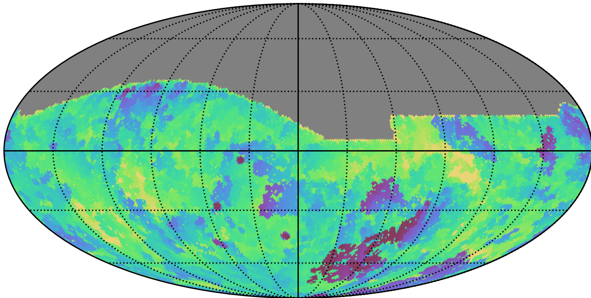
weather_cloudso35v3.4_10yrs All sky g band: Min fiveSigmaDepth
