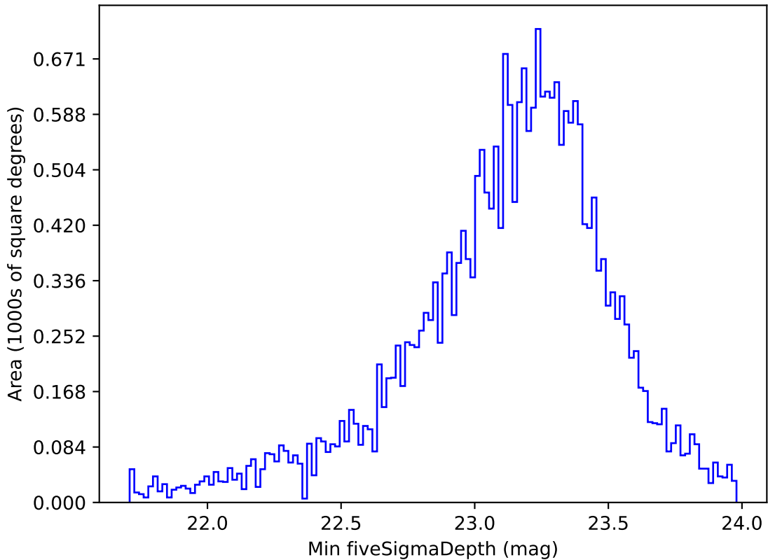
weather_cloudso35v3.4_10yrs All sky g band: Min fiveSigmaDepth
