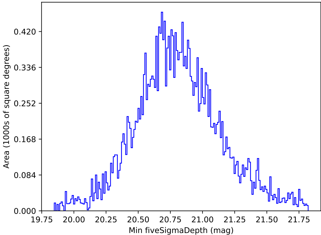
weather_cloudso35v3.4_10yrs All sky all bands: Min fiveSigmaDepth
