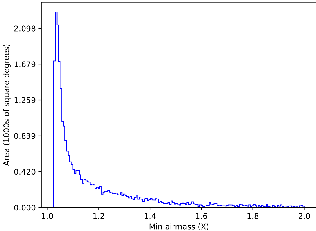
weather_cloudso35v3.4_10yrs Yr 1 z band: Min airmass
