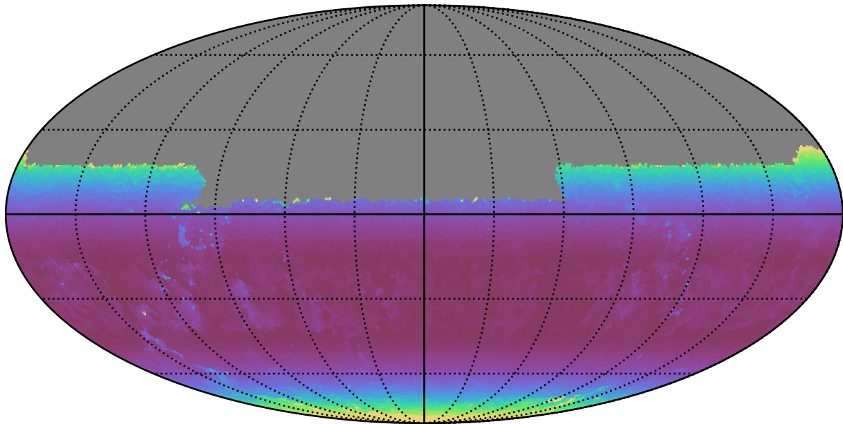
weather_cloudso35v3.4_10yrs Yr 1 y band: Min airmass
