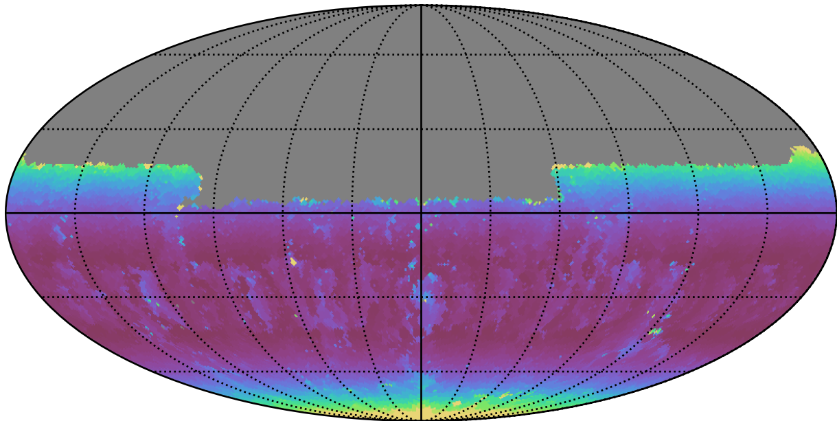
weather_cloudso35v3.4_10yrs Yr 1 u band: Min airmass
