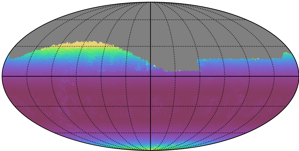
weather_cloudso35v3.4_10yrs Yr 1 r band: Min airmass
