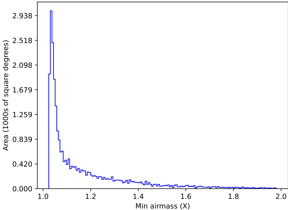
weather_cloudso35v3.4_10yrs Yr 1 r band: Min airmass
