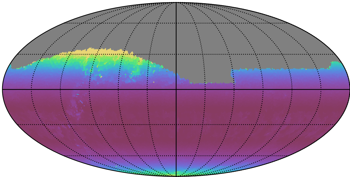
weather_cloudso35v3.4_10yrs Yr 1 i band: Min airmass
