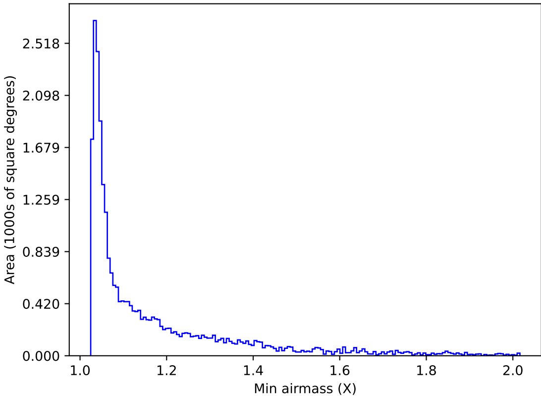
weather_cloudso35v3.4_10yrs Yr 1 i band: Min airmass
