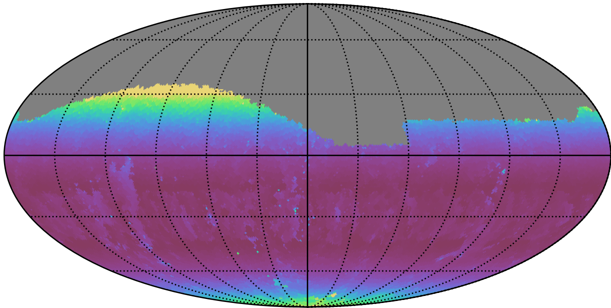
weather_cloudso35v3.4_10yrs Yr 1 g band: Min airmass
