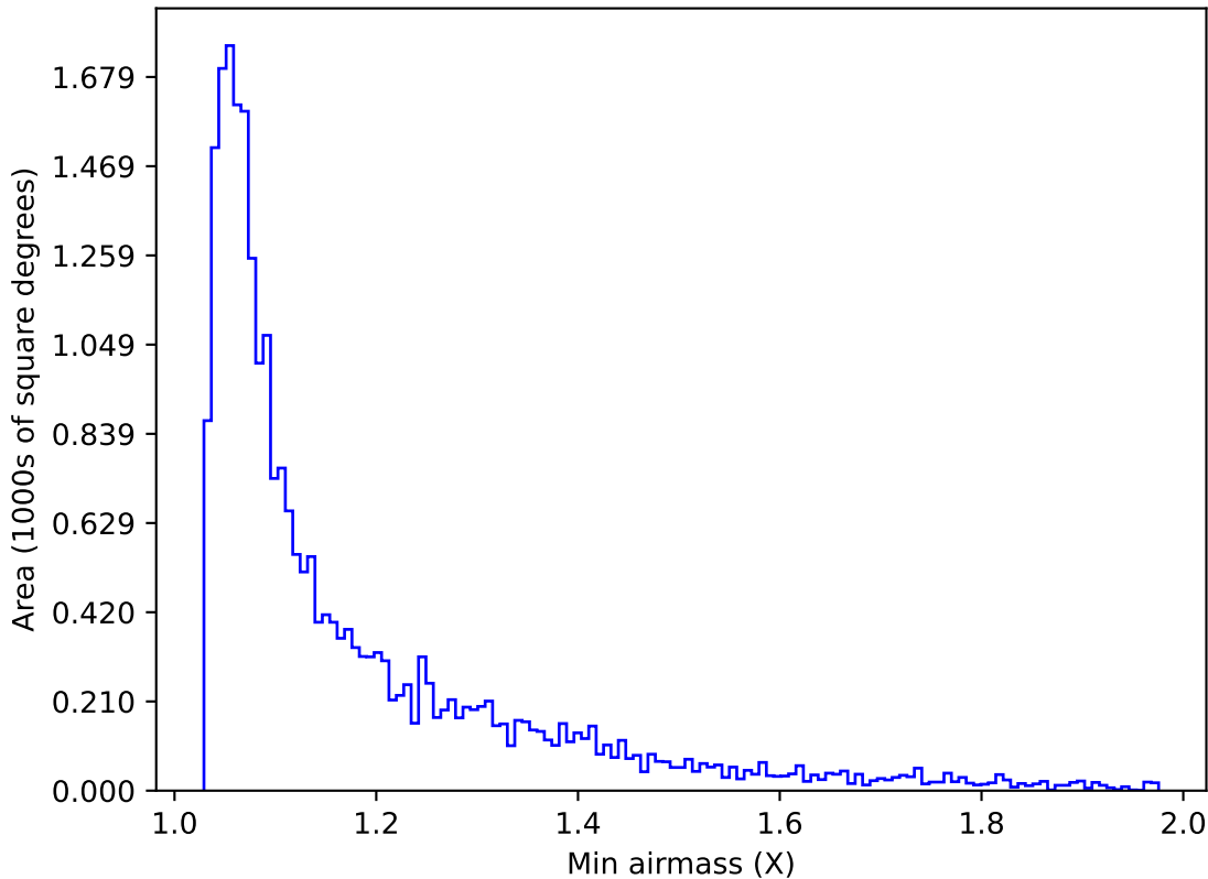
weather_cloudso35v3.4_10yrs Yr 1 g band: Min airmass
