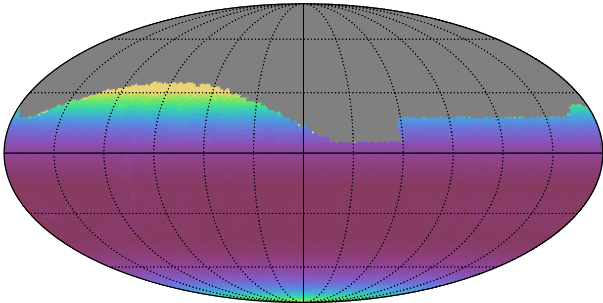
weather_cloudso35v3.4_10yrs Yr 1 all bands: Min airmass
