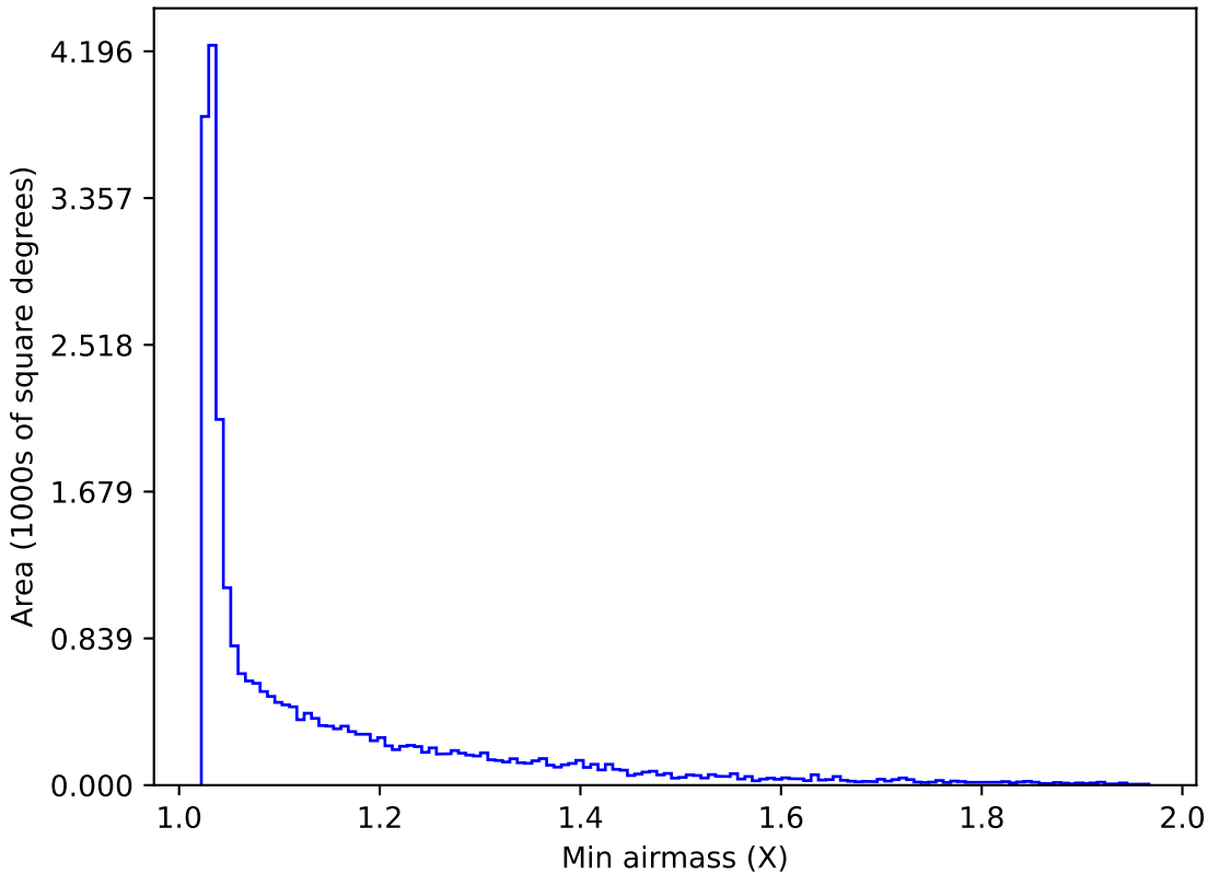
weather_cloudso35v3.4_10yrs Yr 1 all bands: Min airmass
