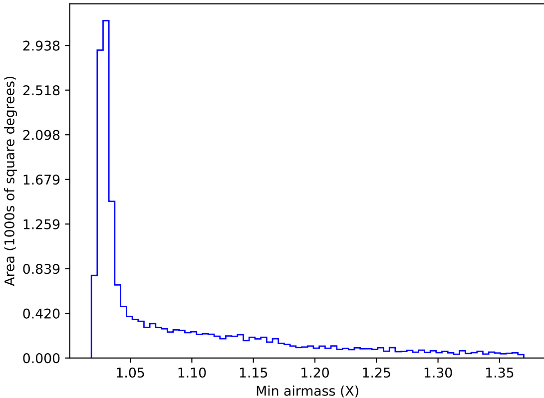
weather_cloudso35v3.4_10yrs WFD z band: Min airmass
