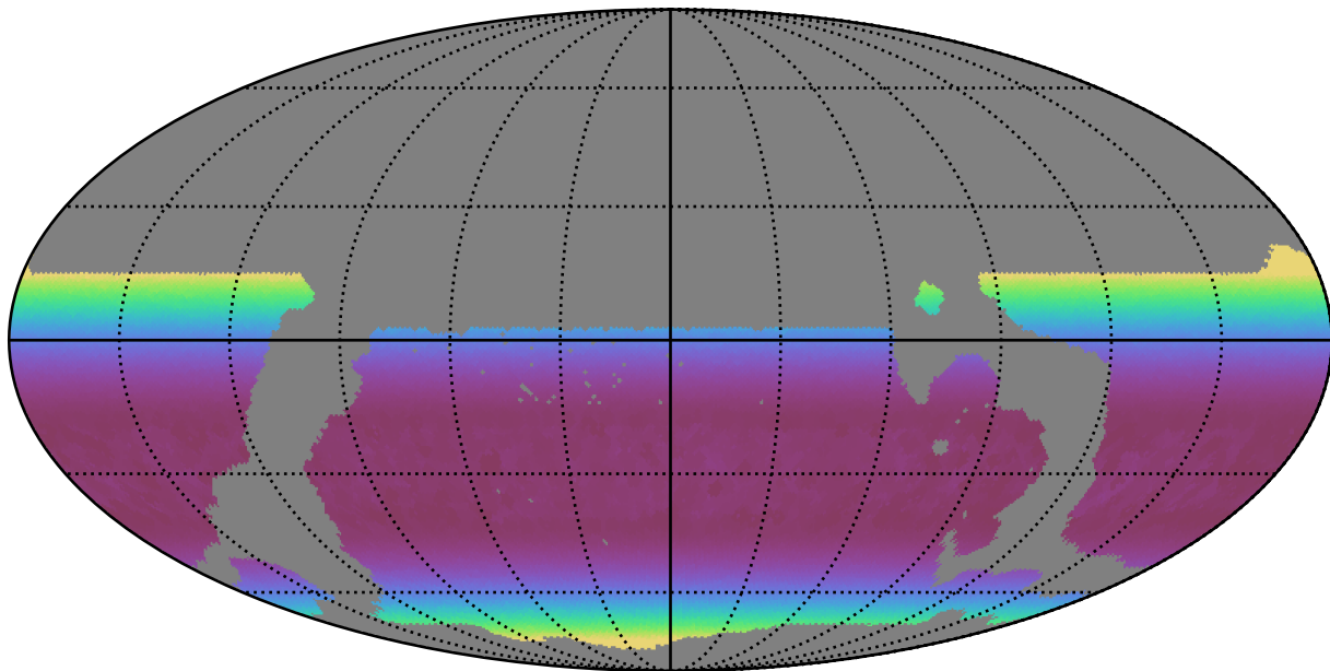
weather_cloudso35v3.4_10yrs WFD r band: Min airmass
