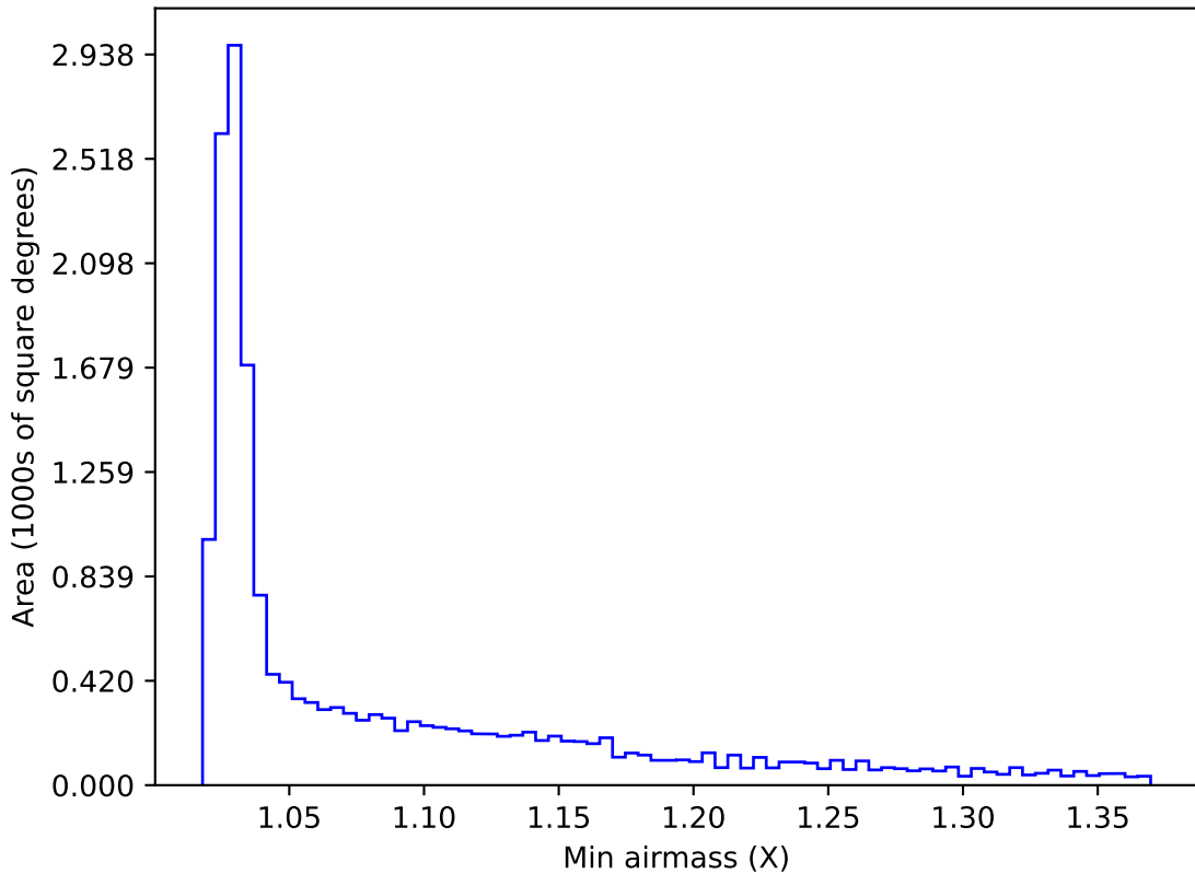
weather_cloudso35v3.4_10yrs WFD i band: Min airmass
