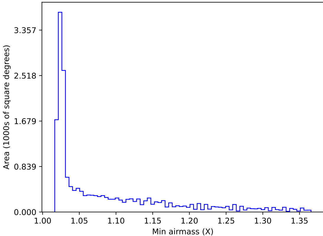
weather_cloudso35v3.4_10yrs WFD all bands: Min airmass
